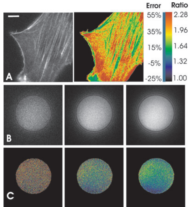
Fig. 3. Noise-induced systematic error in fluorescence ratio imaging. Image of an NIH3T3 cell stained with Alexa-488 phalloidin is acquired at an overall SNR \sim 2.2 (A, left panel). Systematic error at each pixel, if this image were used as the denominator image in ratio imaging, is calculated according to the estimated local SNR and the theoretical curve shown in Fig. 2(A), and rendered in pseudo-colour (A, right panel). Colour-coding of the relative error is indicated in the colour scale (numbers under 'Error'). The blue bar to the left of the scale indicates the colour for 0% error. Bar, 5 \mu\text{m} . The effect of noise in actual ratio imaging is demonstrated by taking the ratio between images of a 5.68- \mu\text{m} polychromatic bead acquired with a GFP (numerator image; not shown) or a YFP (denominator image; B) filter set. The YFP images have an SNR of 2.6 (left), 6.1 (middle), and 11 (right), respectively, in the bead area. Ratio image is rendered in pseudo-colour (C), as indicated in the colour scale (numbers under 'Ratio').
